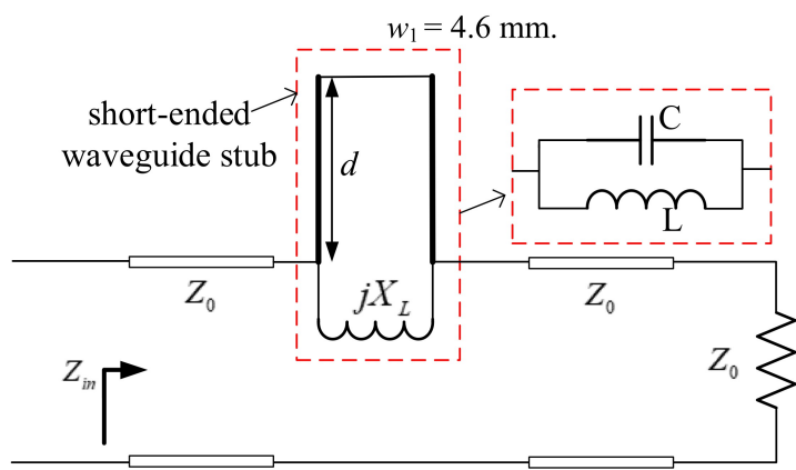
Fig. 3. Equivalent circuit of the SSL with a short-ended waveguide stub.
