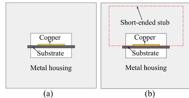
Fig. 1. Cross section of (a) SSL filter with and (b) short-ended stub in the metal housing.
