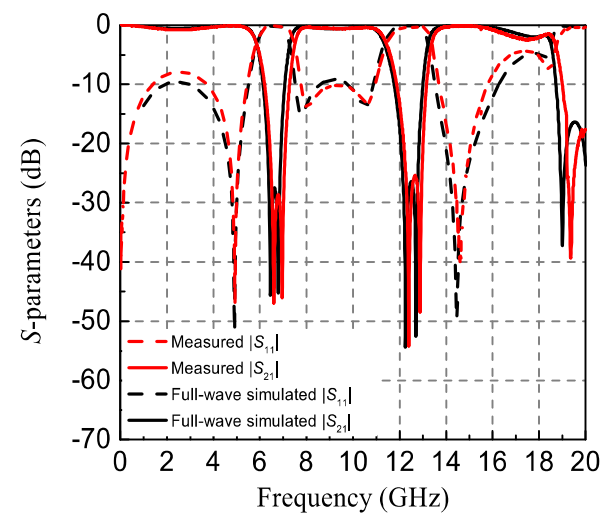
Fig. 10. Measured and simulated S -parameters of the DBBSF.
