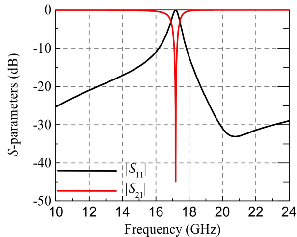
Fig. 4. Full-wave simulated S -parameters of the SSL with a short-ended waveguide stub.
