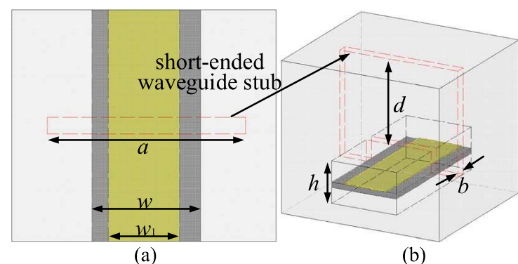
Fig. 2. Geometry of the SSL with a short-ended waveguide stub. (a) Top view and (b) 3-D view with a = 12 mm, b = 1 mm, d = 8 mm, h = 4 mm, w = 6.6 mm, and w_1 = 4.6 mm.
