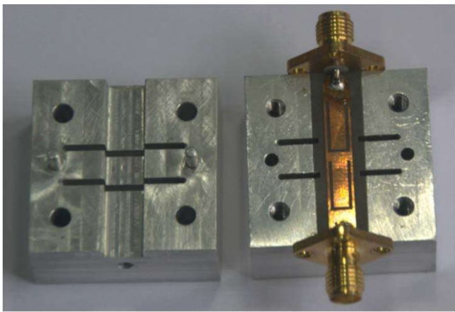
Fig. 9. Photograph of the DBBSF with U-shaped slots.
