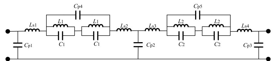
Fig. 6. Equivalent circuit of the BSF.
