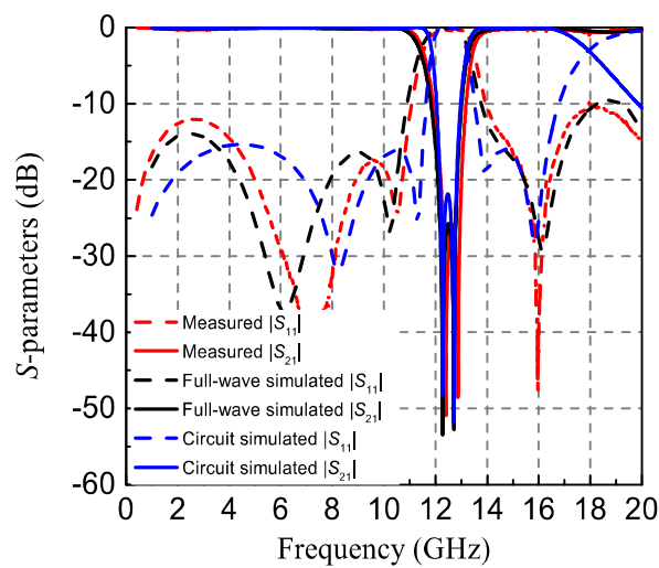
Fig. 7. Measured and simulated S -parameters of the BSF.
