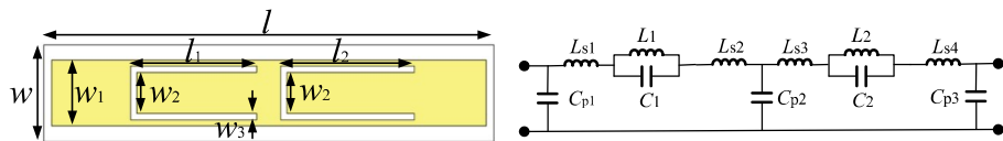
Fig. 8. Geometry of the two U-shaped slots with w_2 = 2.7 mm, w_3 = 0.5 mm, l_1 = 8.4 mm, and l_2 = 8.9 mm.
