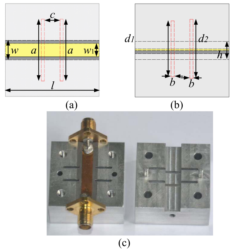
Fig. 5. Structure of the BSF. (a) Top view, (b) side view, and (c) photograph of the fabricated filter with a = 20 mm, b = 1 mm, d_1 = 18 mm, d_2 = 19 mm, c = 5 mm, w = 6.3 mm, w_1 = 4.3 mm, h = 5.8 mm, and l = 30 mm.
